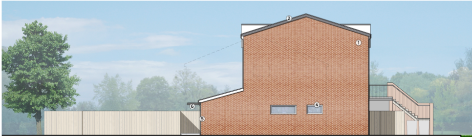
Side Elevation for Plot 3
