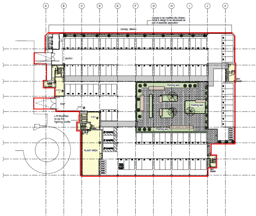
Proposed second floor (refurbishment of existing levels)
