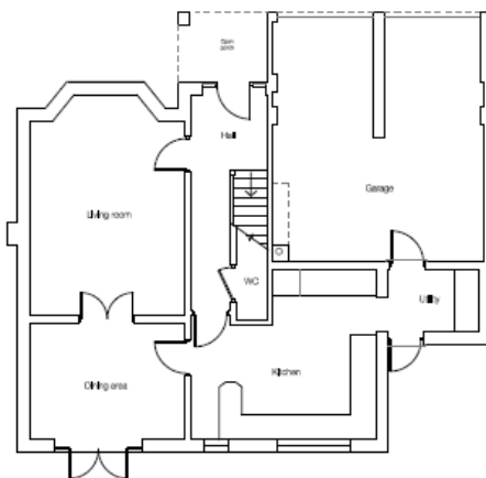
Existing Ground Floor Plan Scale 1:50 @A1 0 1 2 3 4 5m LINEAR SCALE
