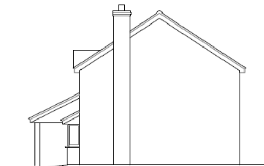
Existing Side (S) Elevation Scale 1:50 @A1
