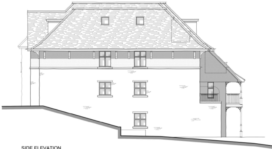
SIDE ELEVATION
